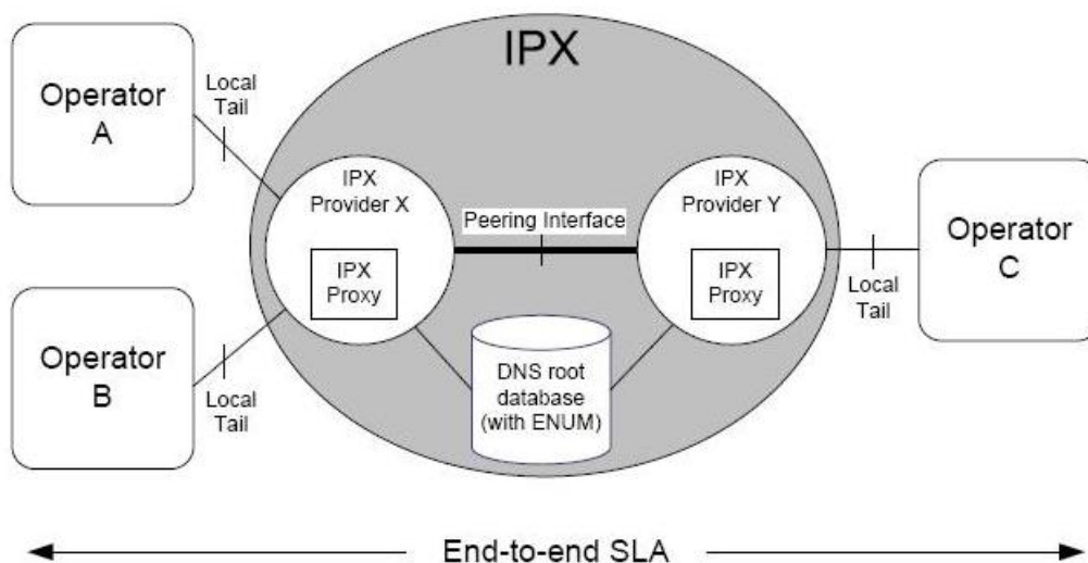
Figure 3: High-Level View of IPX (from IR.34)
