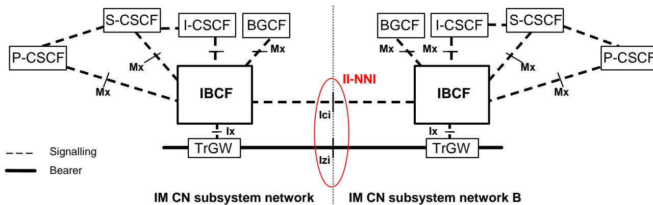
Figure 1: IMS interconnection using Ici & Izi Interfaces (from 3GPP TS 23.228)
