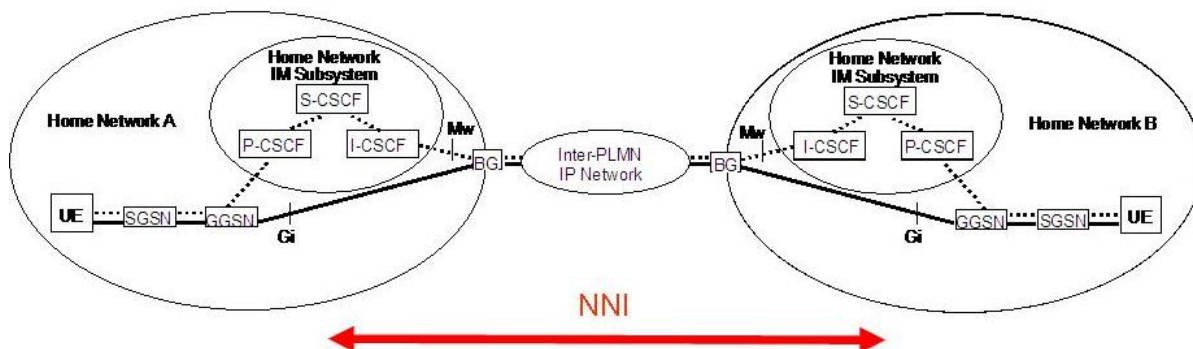
Figure 2: Mw & Gi Interfaces (simplified example missing e.g. FW nodes)
